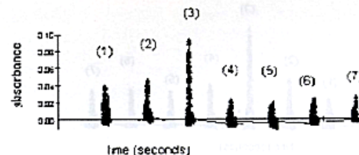
Fig. 2 Absorbance versus run time for silica determination with (1) 2 ppm (2) 5 ppm (3) 10 ppm standards, (4) (5) and (6) (7) were obtained from water samples. Results are in duplicates
