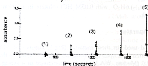
Fig.4 Absorbance versus run time for iron standards with concentration of (1) 0.5 ppm (2) 5 ppm (3) 10 ppm (4) 30 ppm (5) 50 ppm.
