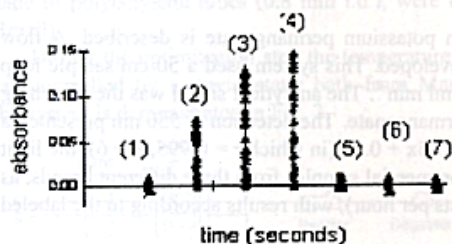
Fig 5 Absorbance versus run time for ammonia determination with (1) 0.5 ppm (2)10 ppm (3) 20 ppm (4)30 ppm standards, (5) (6) (7) were obtained from water samples (triplicates).
