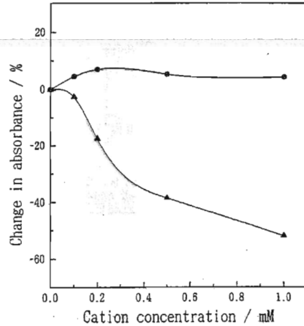
Fig. 7. Effect of foreign cations on the determination of cyanide: (●) \text{Ca}^{2+} , (▲) \text{Zn}^{2+} . Cyanide concentration was 0.1 mM.
