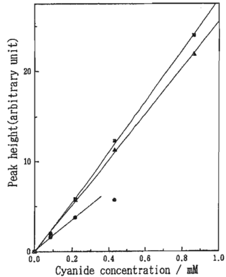
Fig. 5. Effect of thiosulfate concentration on peak height; (●) 2 mM, (▲) 5 mM, (▼) 10 mM S 2 O 3 2- . Cyanide samples were injected into the FIA system with the immobilized enzyme reactor.
