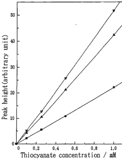
Fig. 4. Effect of iron(Ⅲ) nitrate concentration on peak height; (●) 10 mM, (▲) 30 mM, (▼) 50 mM Fe 3+ . Thiocyanate samples were injected into the FIA system without the immobilized enzyme reactor.
